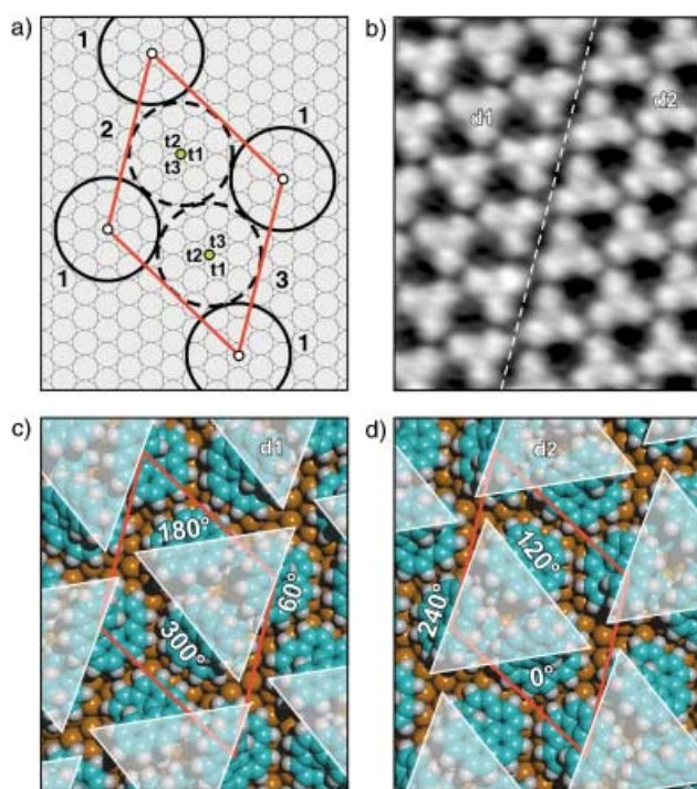
Figure 5. Molecular modeling results compared to STM results of the 3-structure at saturated monolayer coverage. a) Adsorption sites within the unit cell considered for the calculations. b) STM image of a domain boundary (dashed line) between the two rotational domains d1 and d2. c) and d) The two lowest total-energy configurations as determined from the calculations. White semi-transparent triangles highlight the topmost parts of the molecules that are imaged brightest. Both geometries are in excellent agreement with the observed d1 and d2 domain structures.
