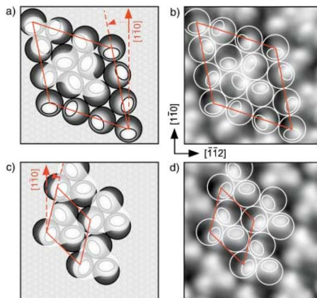
Figure 4. Structure models for the ( M )-heptahelicene 6&3-molecule cluster (a and b) and the ( M )-heptahelicene 3-molecule cluster structures (c and d) based on a hexagonal packing of the molecules and systematically varying azimuthal orientations. The model structures are superimposed on the corresponding STM images in (b) and (d).
