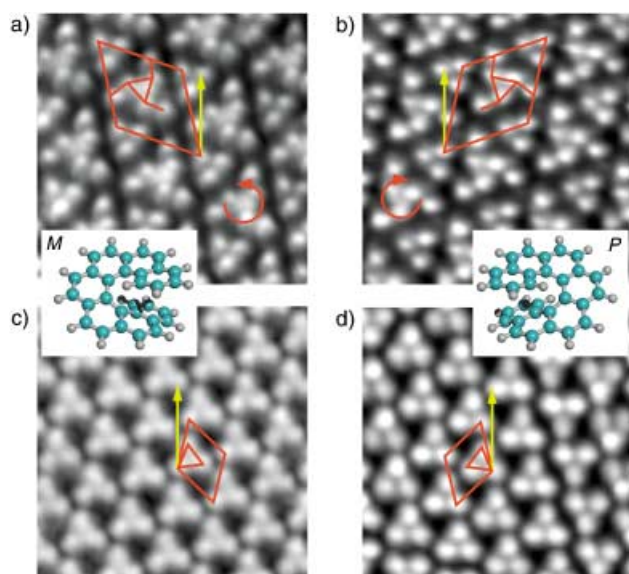
Figure 2. High-resolution STM images of ( M )- and ( P )-[7]H structures (10 nm × 10 nm). a) ( M )-[7]H at \theta = 0.95 . b) ( P )-[7]H at \theta = 0.95 . c) ( M )-[7]H at \theta = 1 . d) ( P )-[7]H at \theta = 1 . The ( M )- and ( P )-[7]H structures are mirror images of each other. Unit cells and their basic building blocks are outlined by red lines, the [1\bar{1}0] surface direction is indicated by the yellow arrows.
