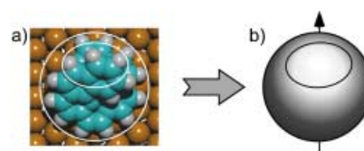
Figure 3. Topographic model used for the interpretation of the observed STM images: The [7]H molecule, as adsorbed on Cu(111) (a), is approximated by a disk with a bright protrusion at the topmost part of the molecule (b). The azimuth of a protrusion pointing towards the “12-o'clock” direction is defined as 0^\circ .
